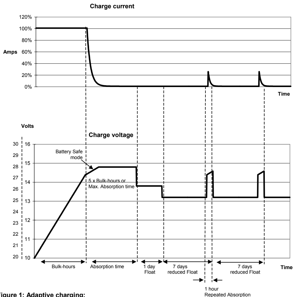
Figure 1: Adaptive charging:
